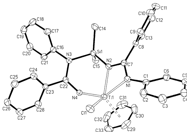
Figure 1. ORTEP drawing (30% probability level) of the molecular structure of compound 1 . Hydrogen atoms are omitted for clarity.
