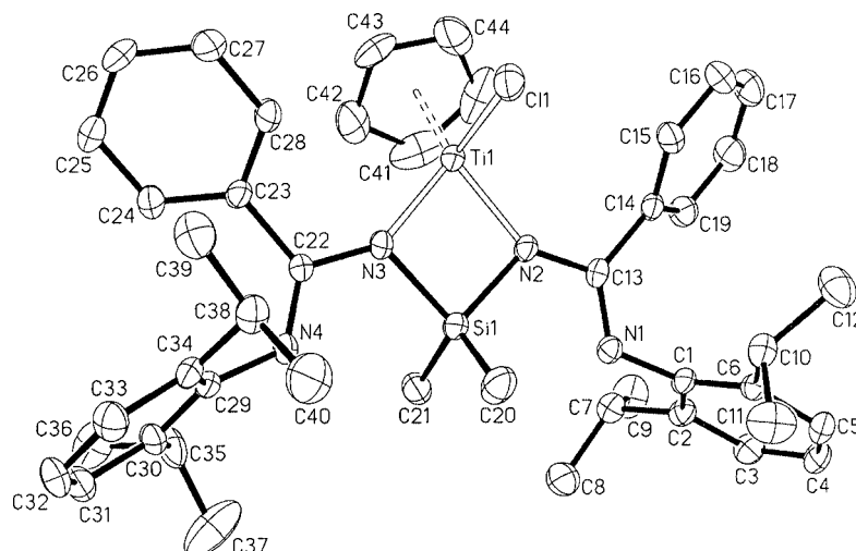
Figure 2. ORTEP drawing (30% probability level) of the molecular structure of compound 3 . Hydrogen atoms are omitted for clarity.
